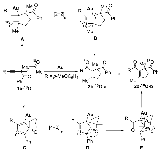
Scheme 4. Isotopic labeling experiment for mechanistic studies.
