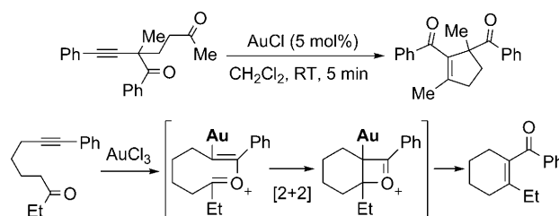
Scheme 3. Gold-catalyzed intramolecular oxygen transfer of alkynylketones.
