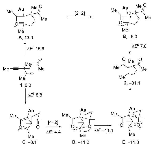
Scheme 5. B2PLYP/6-311+G(d,p)//B2PLYP/6-31G(d) computed reaction profile. Relative energies in kcal mol -1 .
