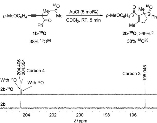
Figure 2. ^{18}\text{O} isotopic experiment and the ^{13}\text{C} NMR spectrum. [a] Determined by MS (ESI). [b] NMR yield.
