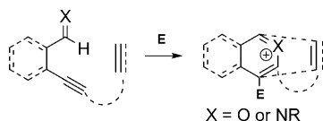
Scheme 1. Formation of oxonium or aminium ions from alkynyl aldehydes or imines.
