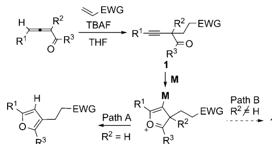
Scheme 2. Formation of furanium ions from propargylic ketones.
