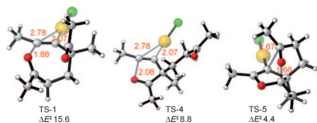
Figure 3. B2PLYP/6-31G(d) transition structures for addition to the alkyne and for [4+2] cyclization.
