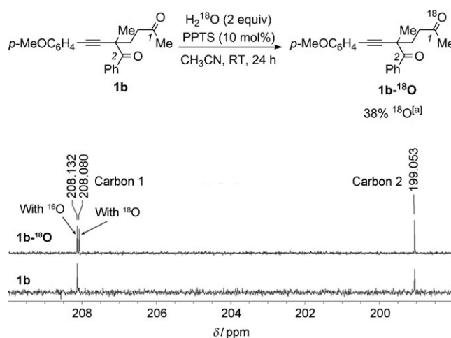
Figure 1. Synthesis of substrate 1b- ^{18}\text{O} and the ^{13}\text{C} NMR spectrum. [a] Determined by MS (ESI).
